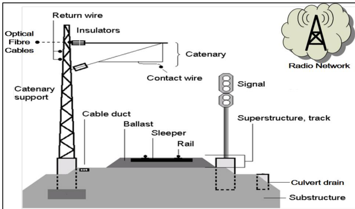
Figure 1: Railway Infrastructure
